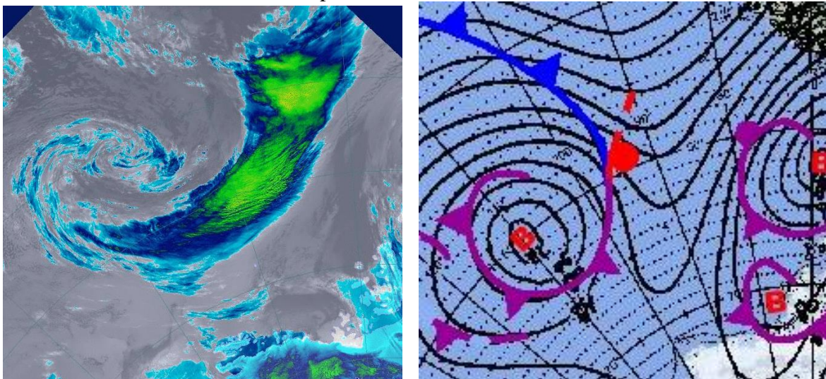
Figure 7- NOAA-18 April-12 satellite pass (left) explained by the Chilean Navy Meteorological Map (right)
