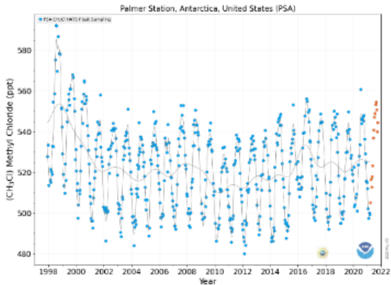
Figure 5- Methyl Chloride (CH 3 CL) Levels at Palmer Station dating back to 1997, one of the Halocarbon and Trace Gases measured at Palmer Station. Orange dots are preliminary data.
